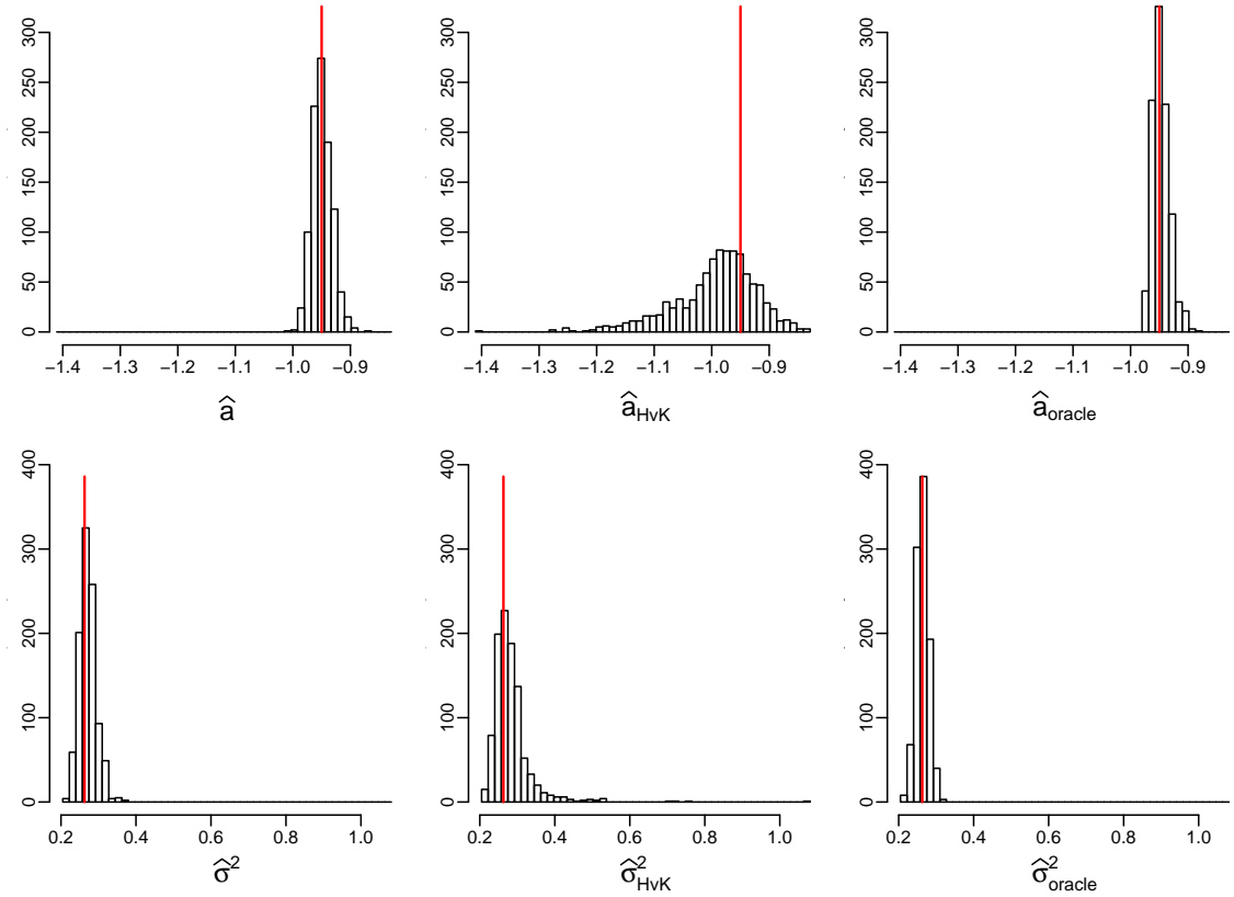
Figure 5: Histograms of the simulated values produced by the estimators \hat{a} , \hat{a}_{\text{HvK}} , \hat{a}_{\text{oracle}} and \hat{\sigma}^2 , \hat{\sigma}_{\text{HvK}}^2 , \hat{\sigma}_{\text{oracle}}^2 in the scenario with a_1 = -0.95 and s_\beta = 1 . The vertical red lines indicate the true values of a_1 and \sigma^2 .
