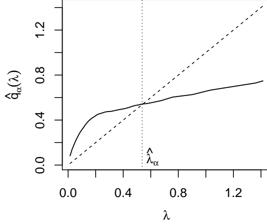
Figure 1: Graphical illustration of the estimator \hat{\lambda}_\alpha . The solid black line is the function \lambda \mapsto \hat{q}_\alpha(\lambda) , the dashed line is the 45-degree line, and the vertical dotted line indicates the value of \hat{\lambda}_\alpha . (The graph was produced by running our method on one of the simulated samples from the Monte Carlo study in Section 5.)
